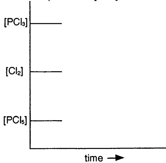
f) increase [\text{PCl}_5]
