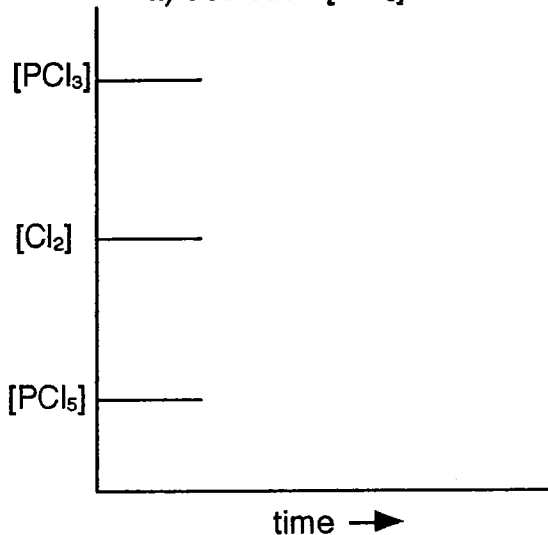
a) decrease [\text{PCl}_3]
