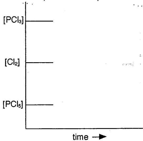
f) increase [\text{PCl}_5]
