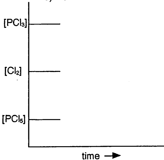
e) increase volume
