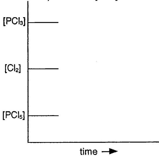
b) decrease [\text{PCl}_5]
